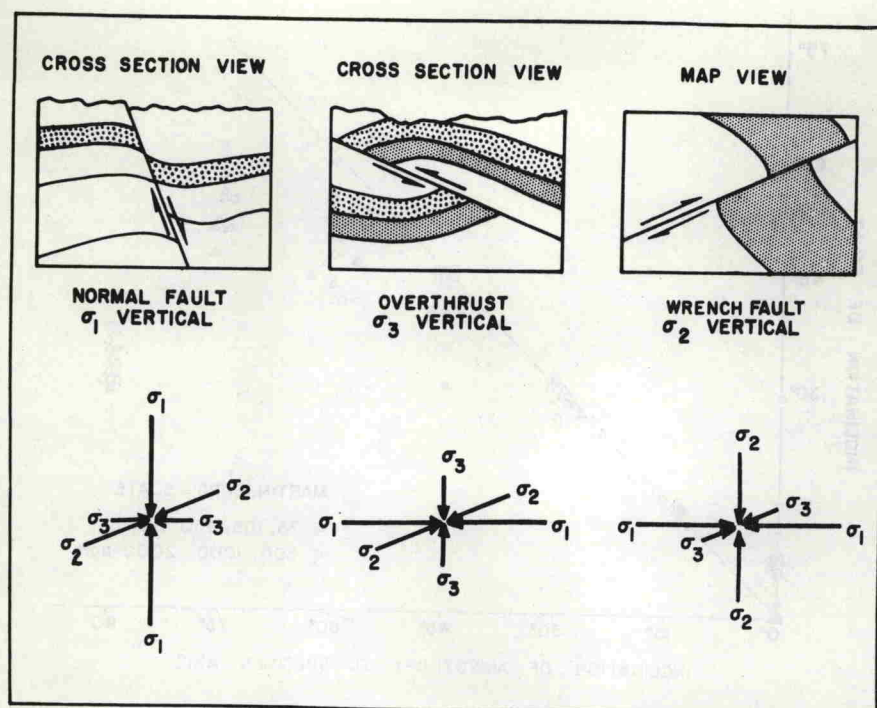
Fig. 10—The orientations of the principal stresses associated with the common fault types (after Anderson, Ref. 68).
