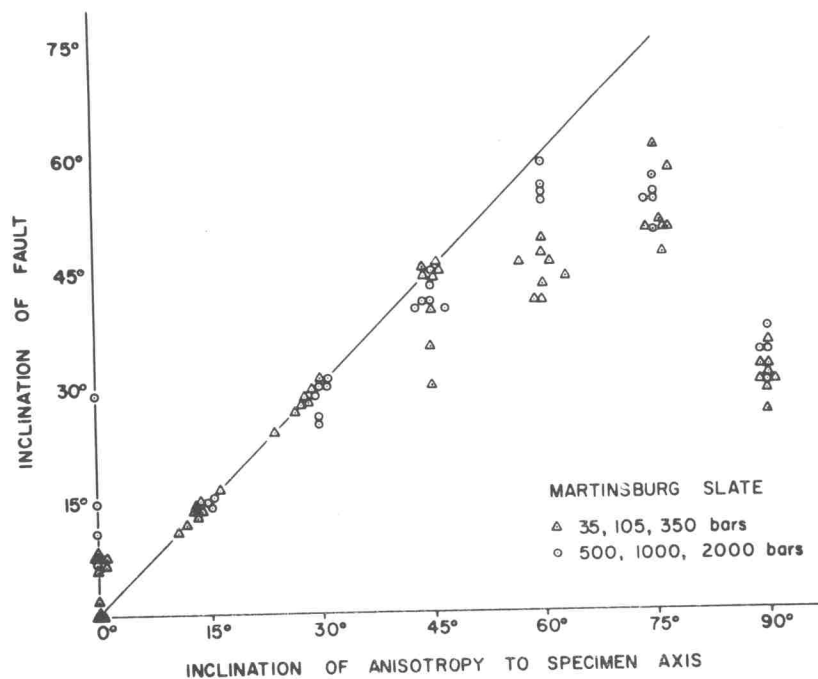
Fig. 9—Effect of cleavage on the angle of faulting, Martinsburg slate (Donath, Ref. 64).
